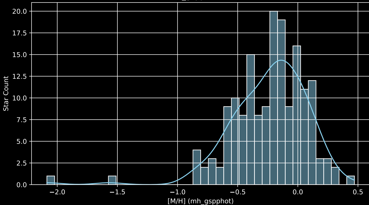
APOGEE DR17 Field: [023+88_MGA [M/H] (mh_gspphot) (n= 168)
