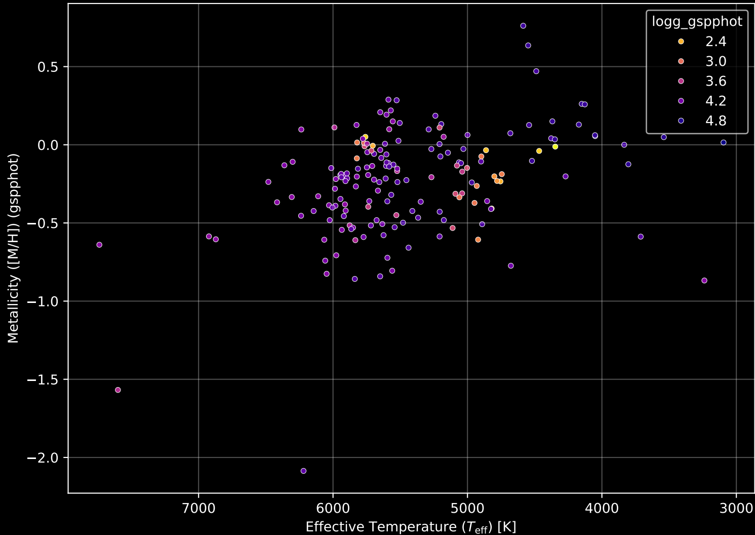
APOGEE DR17 Field: [023+88_MGA] Stellar Population Parameters (n= 170)
