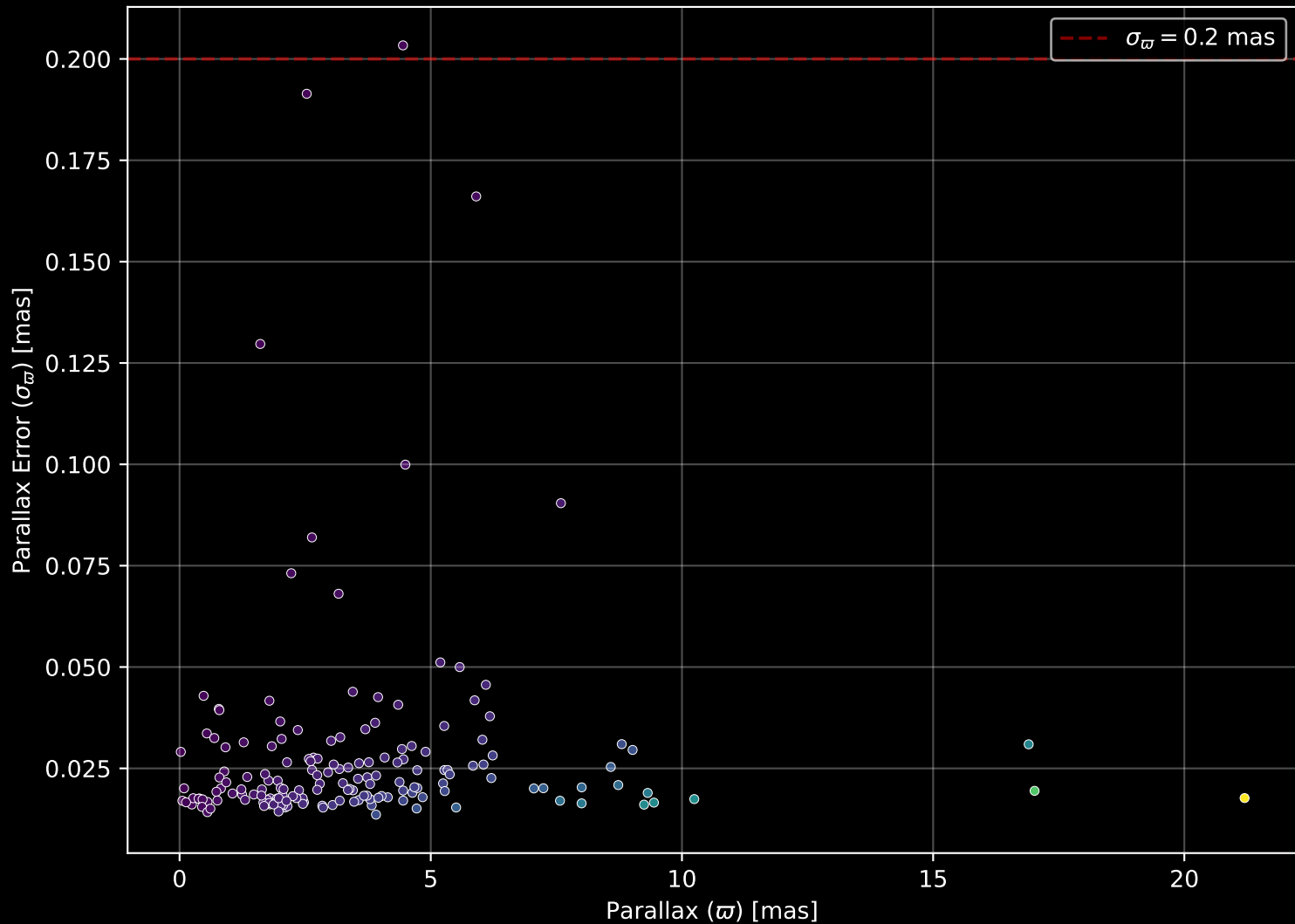
APOGEE DR17 Field: [023+88_MGA] Parallax Quality (n= 170)
