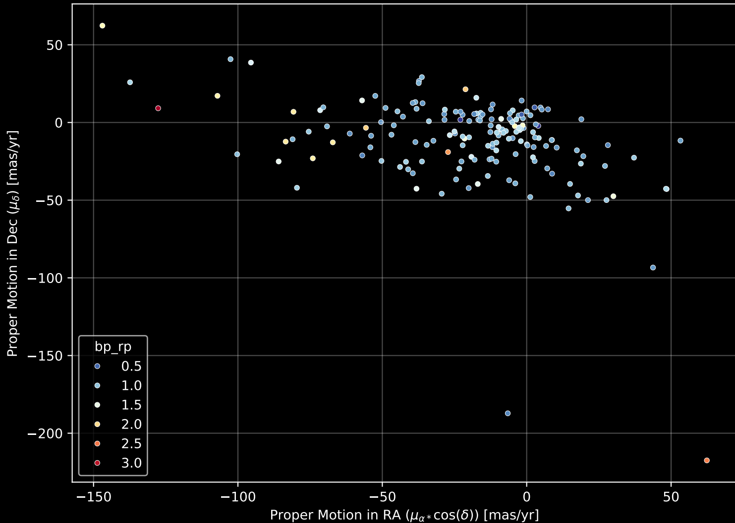
APOGEE DR17 Field: [023+88_MGA] Proper Motion Diagram (n= 170)
