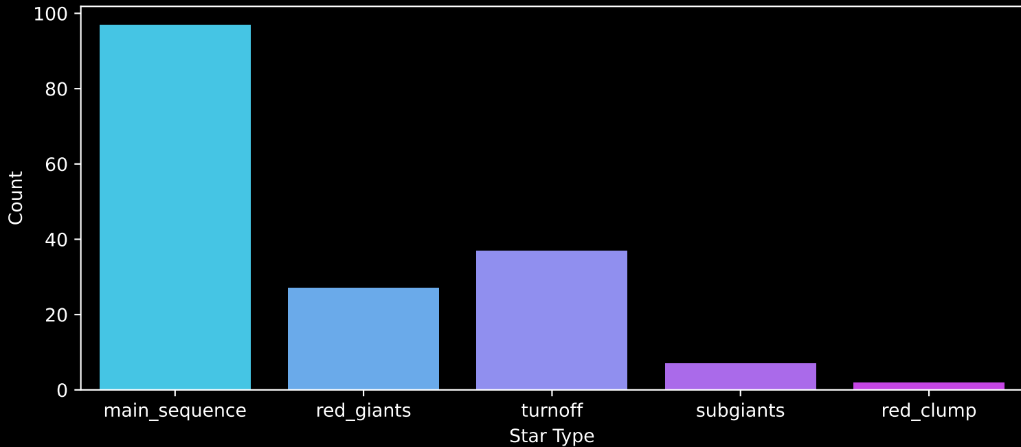
APOGEE DR17 Field: [023+88_MGA] Count plot of Star Type
