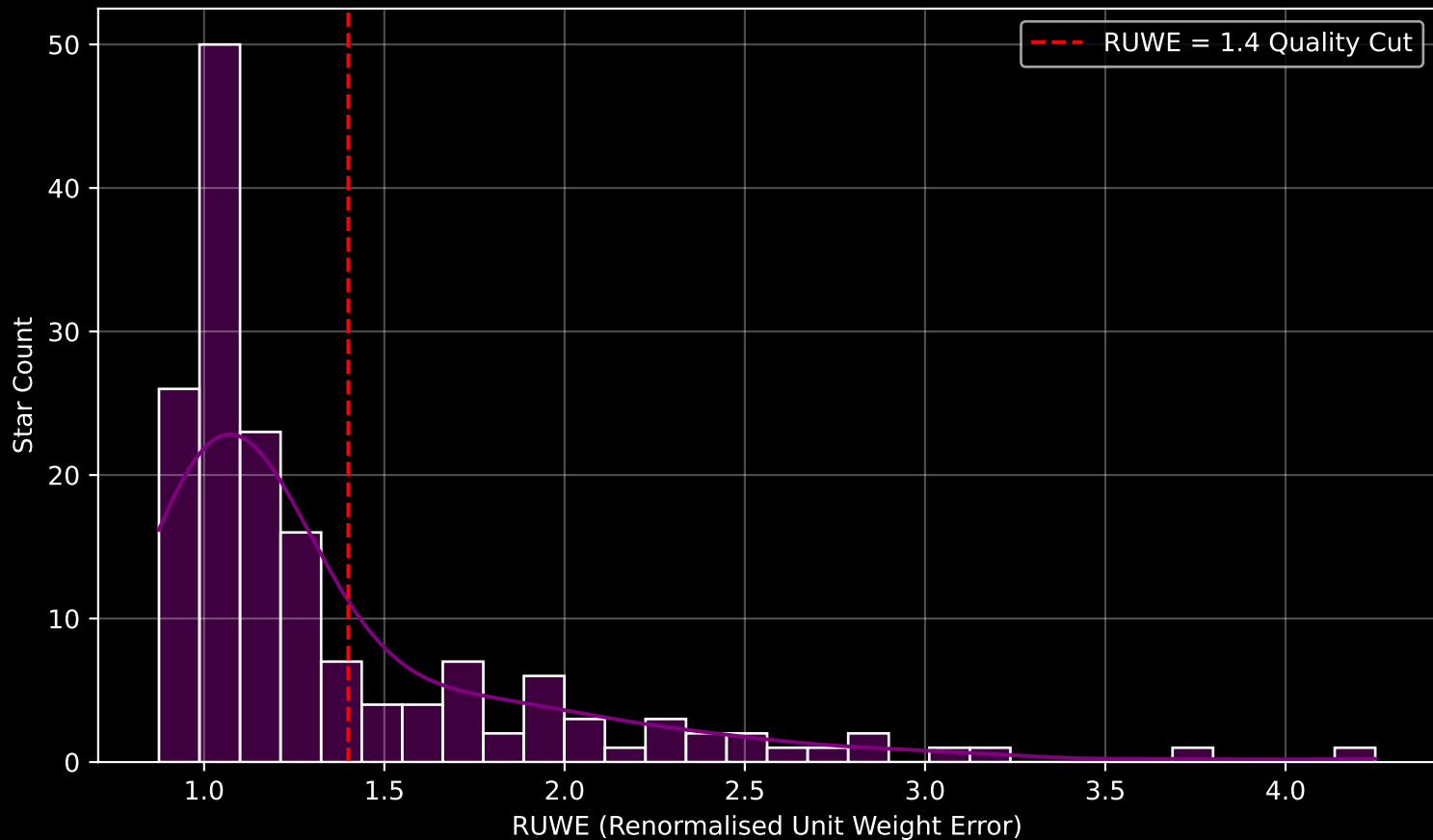
GAPOGEE DR17 Field [023+88_MGA] RUWE Distribution (n= 164)
